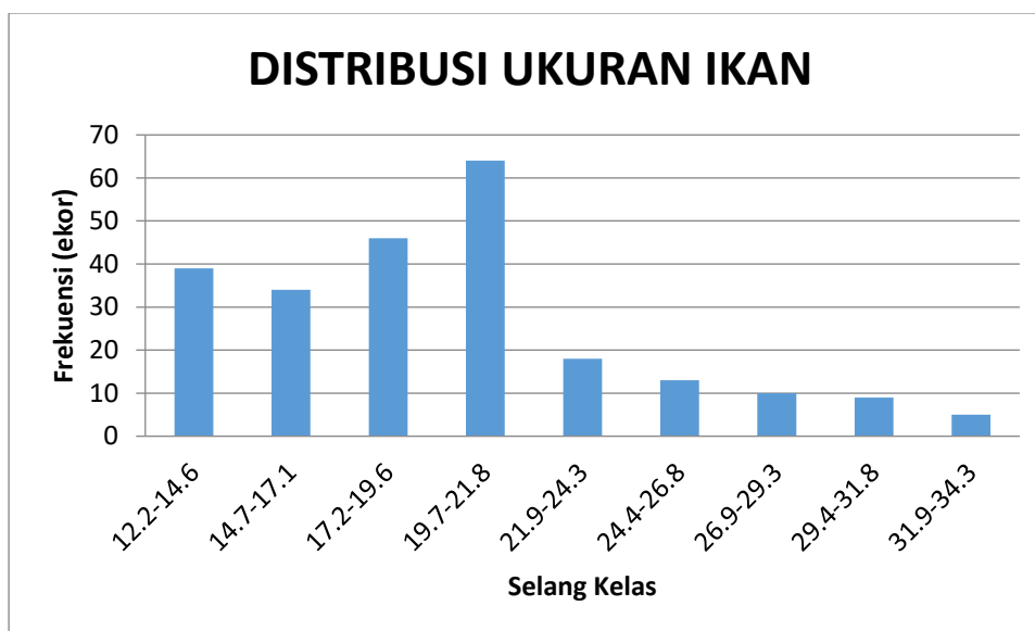
Gambar 2. Distribusi Ukuran Ikan Picture 2. Fish Size Distribution
