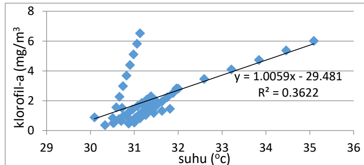
Gambar 6. Grafik hubungan klorofil-a dan suhu permukaan laut. Figure 6. Chlorophyll-a and sea surface temperature relationship graph.
